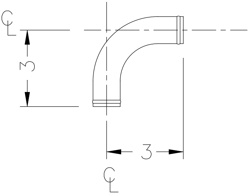
TOP VIEW VENT LINE
