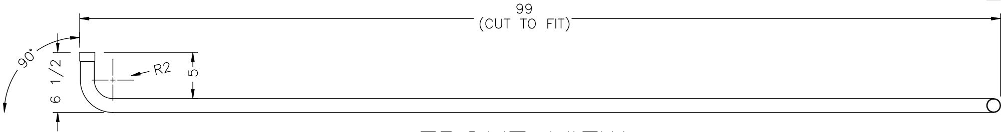
FRONT VIEW
