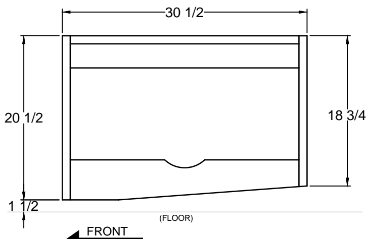
*ARM FRAME DETAIL (SIDE VIEW)
