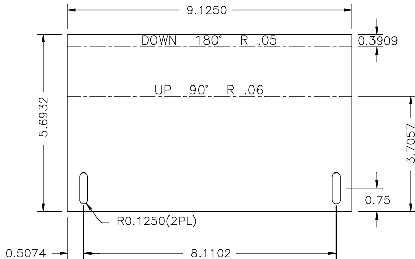
TOP FLAT VIEW
