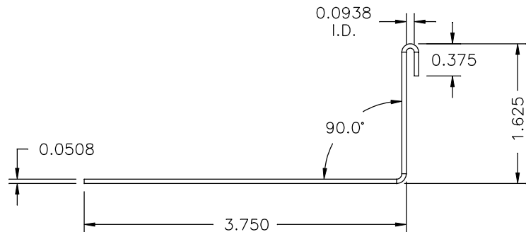
END VIEW AFTER FORMING SCALE 2X
