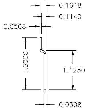
END VIEW AFTER FORMING SCALE 2X
