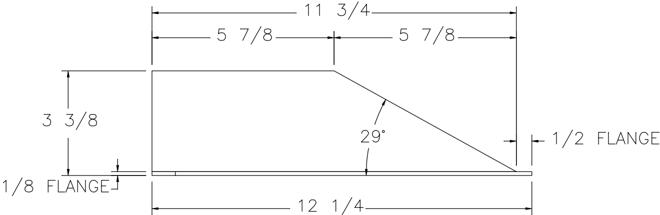
SIDE VIEW
