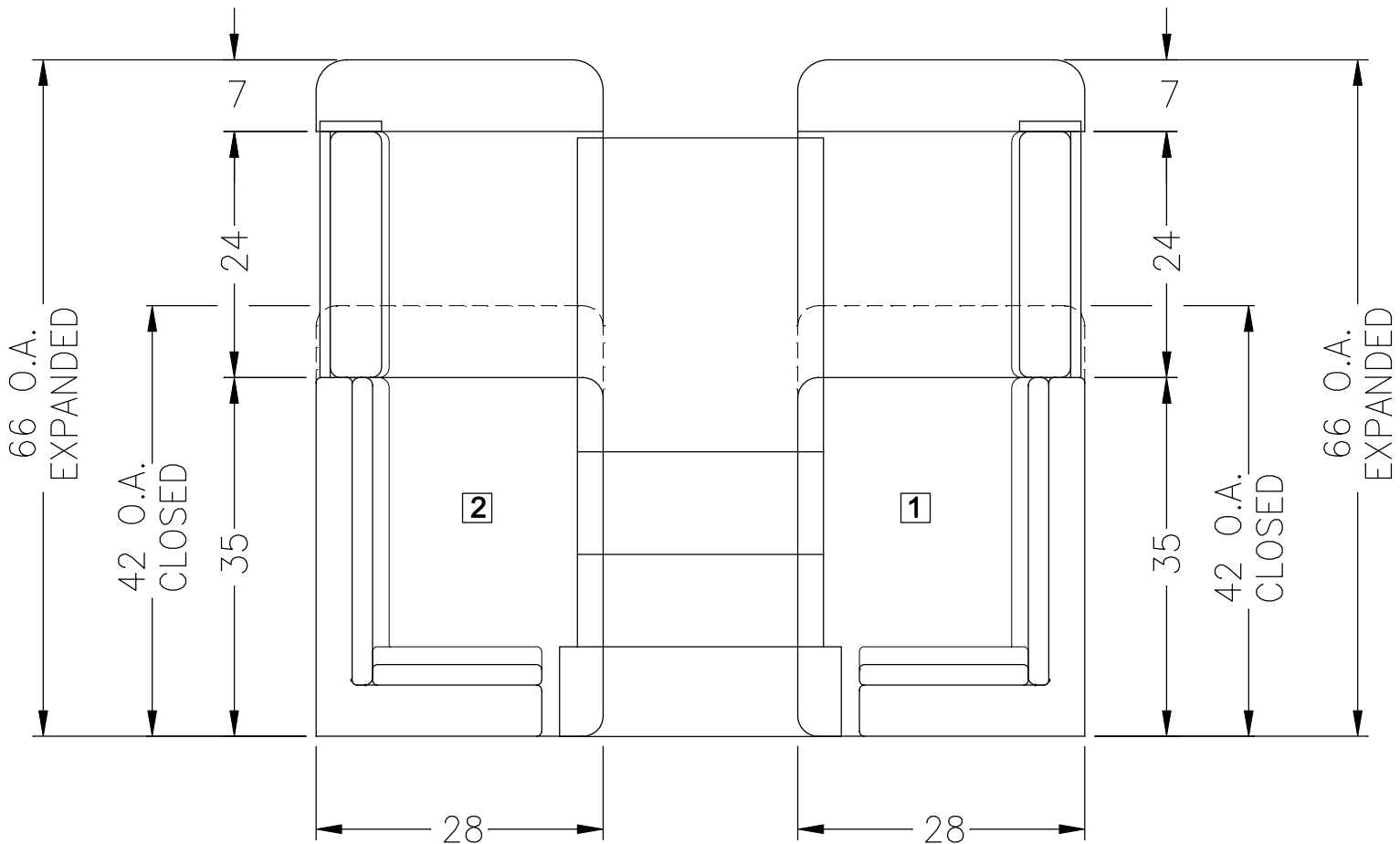
42 EXTENDA BOOTH RT
