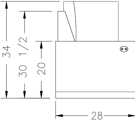
LT SIDE VIEW
