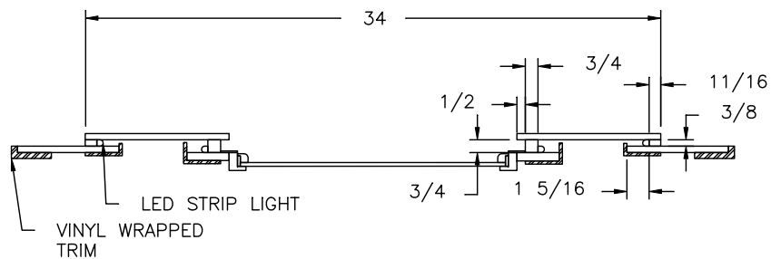
ASSEMBLED CROSS SECTION
