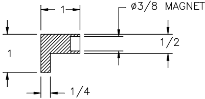
SECTION A-A 4X SCALE
