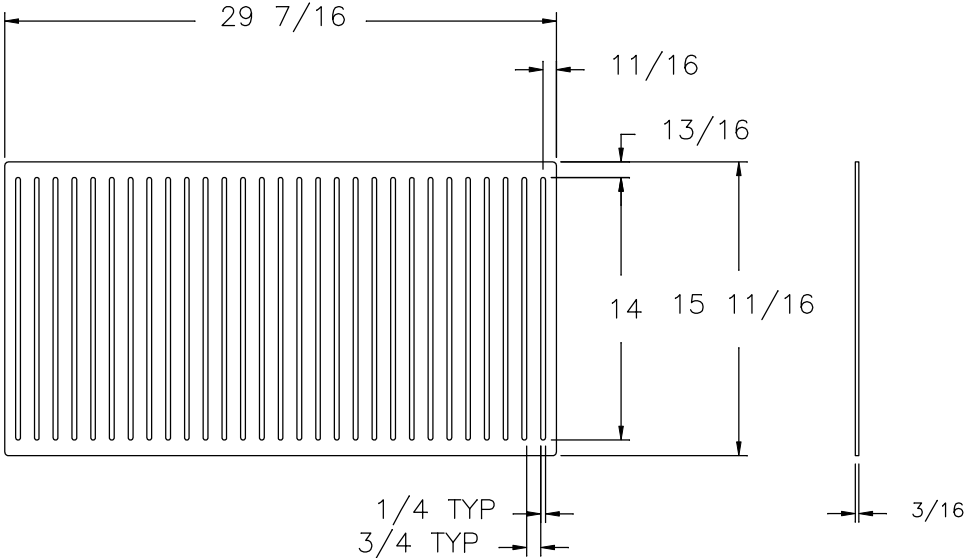
LOUVER PANEL
