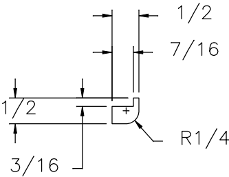
SECTION B-B 4X SCALE
