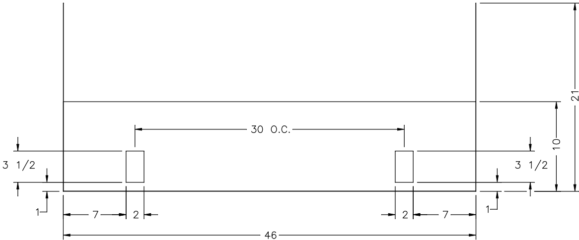
FRONT VIEW
