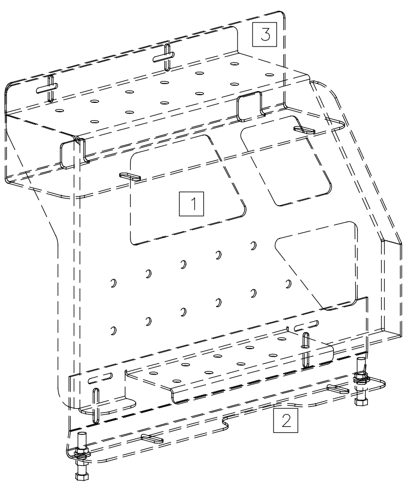
ASSEMBLED VIEW
