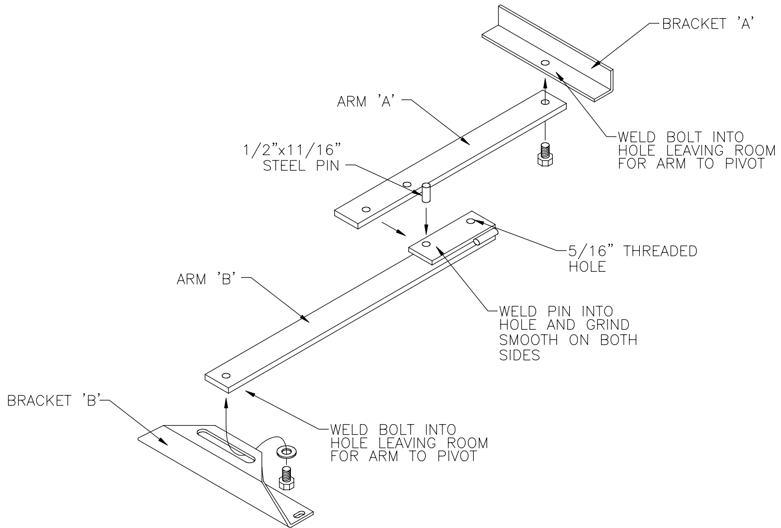
ARM ASSEMBLY
