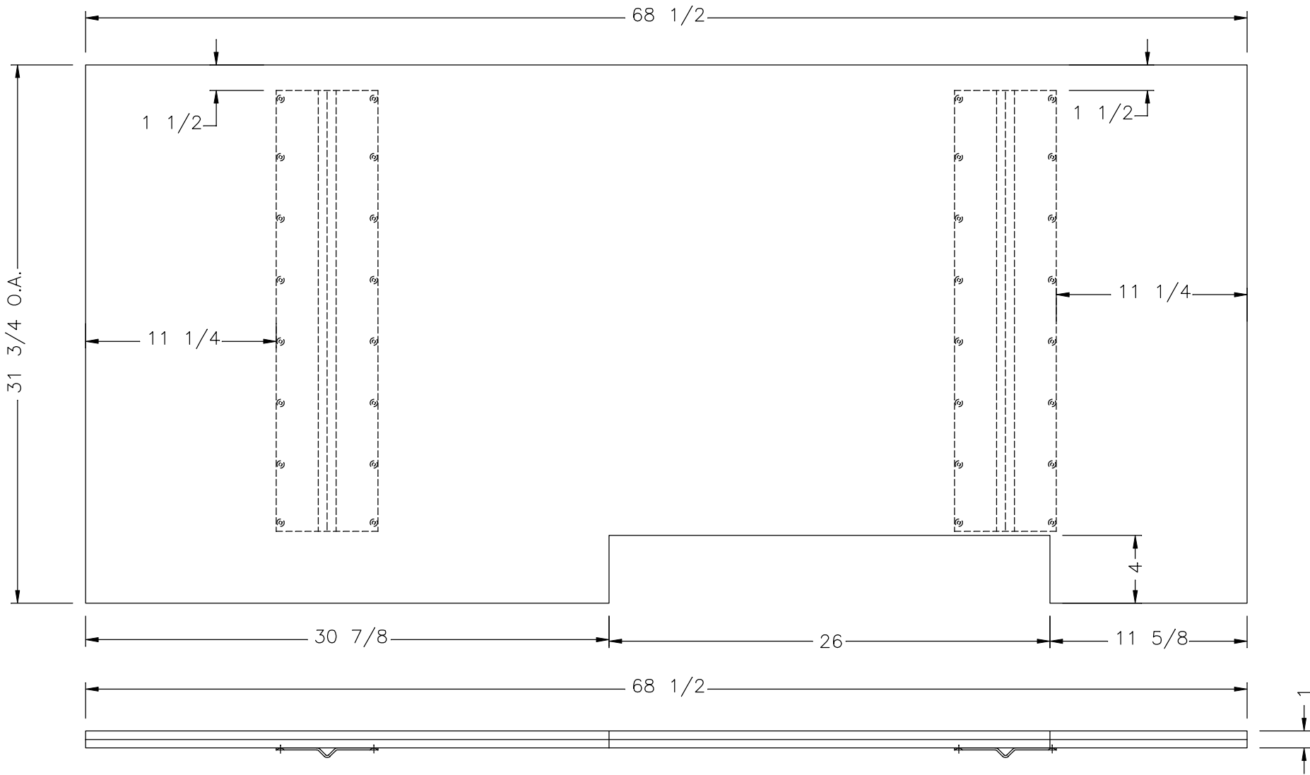
FRONT VIEW
