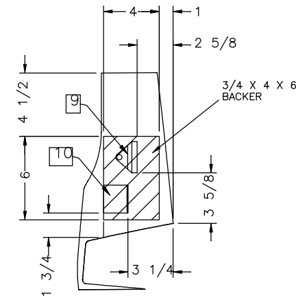
SECTION VIEW C-C (SCALE 4X)
