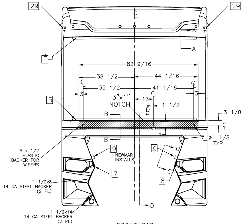
FRONT CAP
