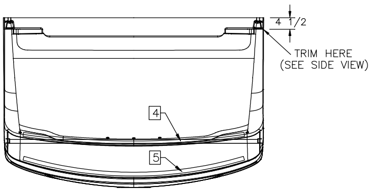
TOP VIEW OF CAP
