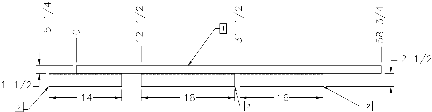
TOP VIEW
