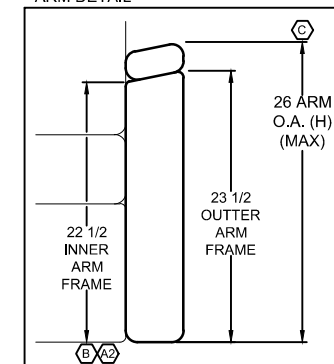
* ARM DETAIL
