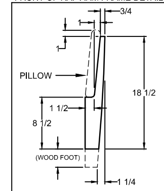
*FRONT OF RAF ARM FRAME DETAIL
