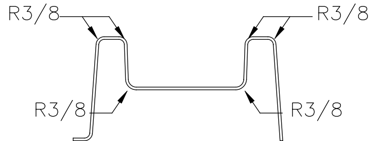
RADII DETAIL OF SECTION (A) AND SECTION (B) (SCALE 2x)
