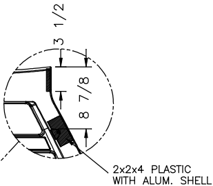
DUTCH STAR REAR ENGINE DOOR GRILL
