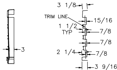
SECTION H-H
