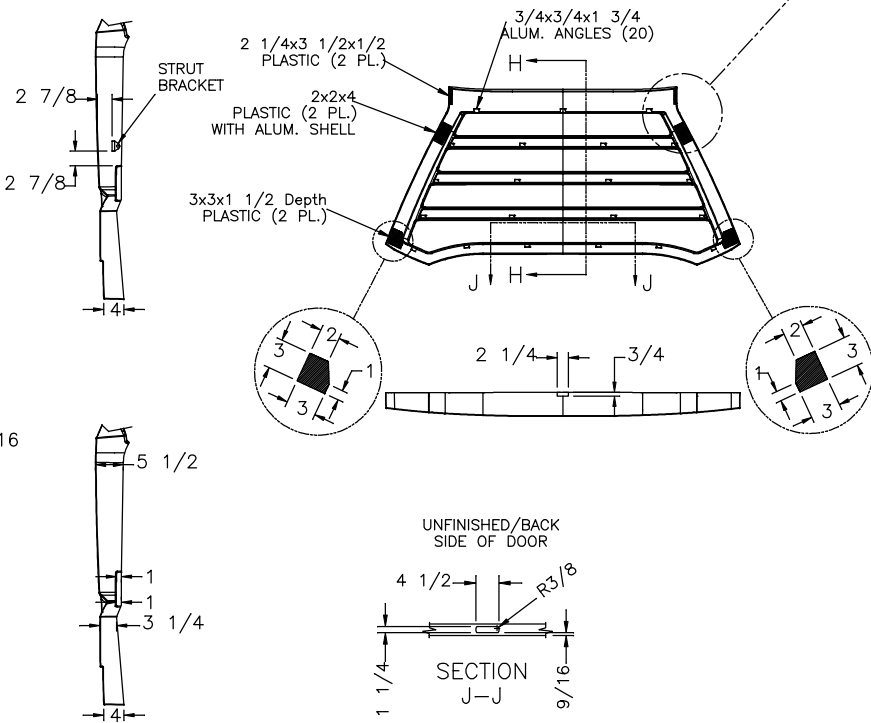
SECTION J-J
