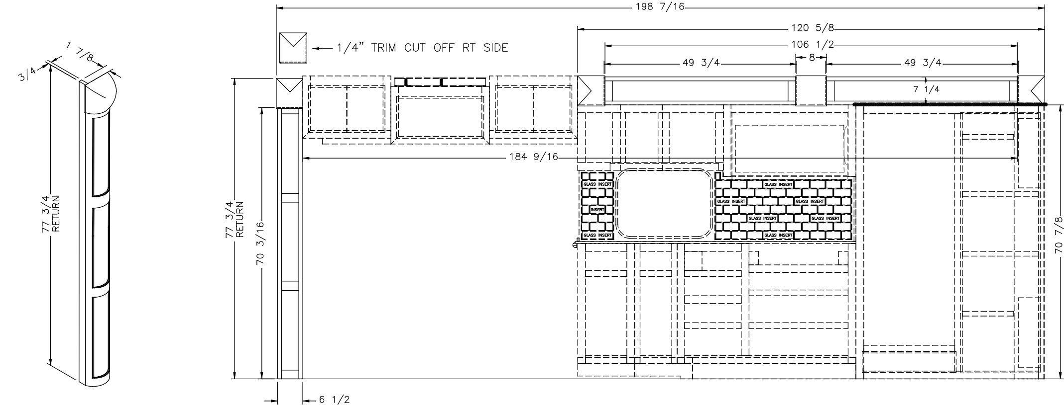
FASCIA RETURN DETAIL
