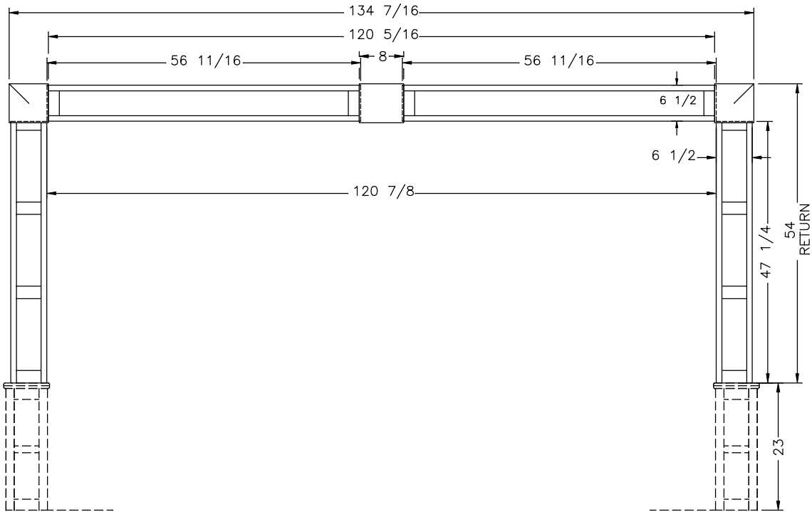
LIVINGROOM S-O FASCIA
