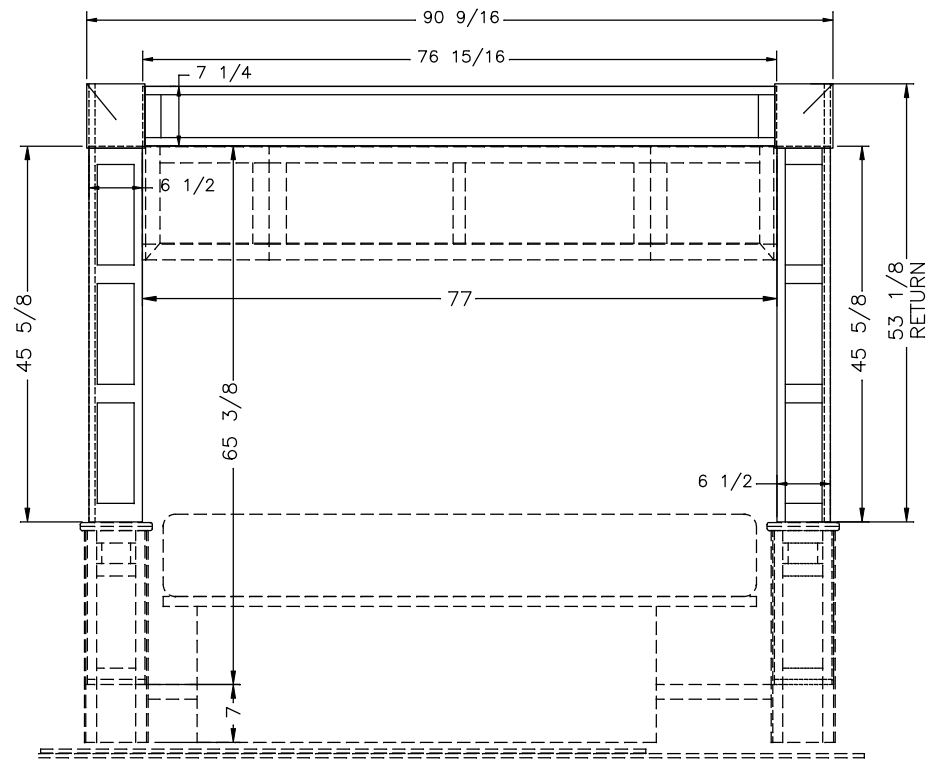
BEDROOM S—O FASCIA
