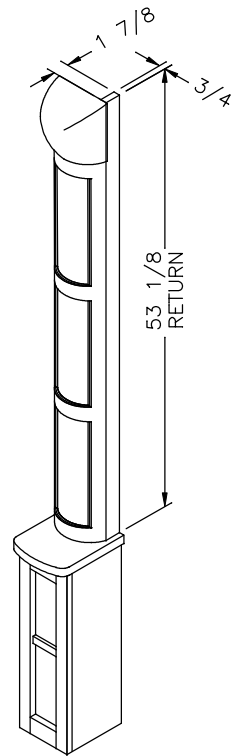
FASCIA RETURN DETAIL
