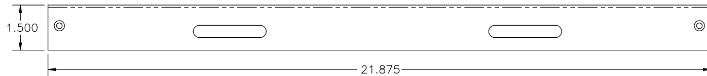
BENT BOTTOM VIEW
