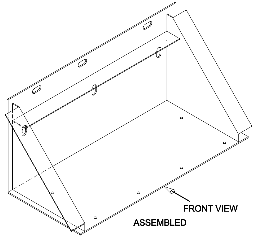
GUSSET PLATE (11 GA.)
