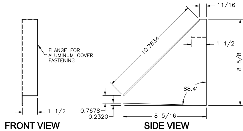
GUSSET PLATE (11 GA.)
