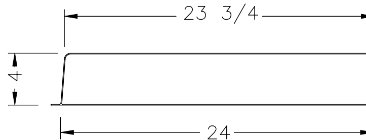
SIDE SECTION (B)
