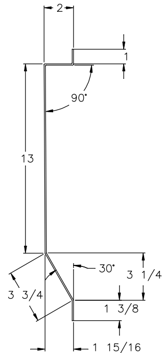
SECTION AA
