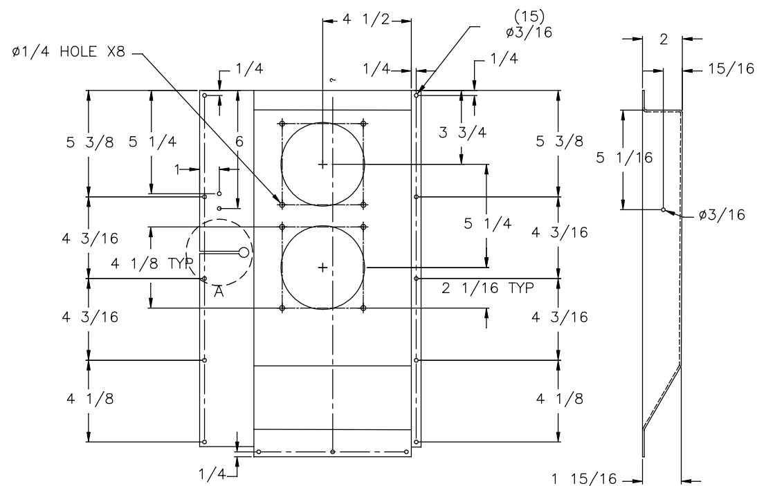
HOLE LOCATIONS
