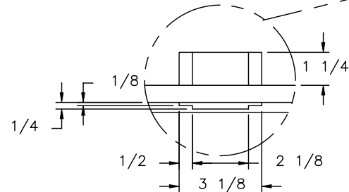
DETAIL B 3/8" PLYWOOD
