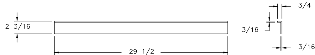
VINYL WRAP DETAILS – INNER EDGE OF DETAIL B 2 EACH REQUIRED
