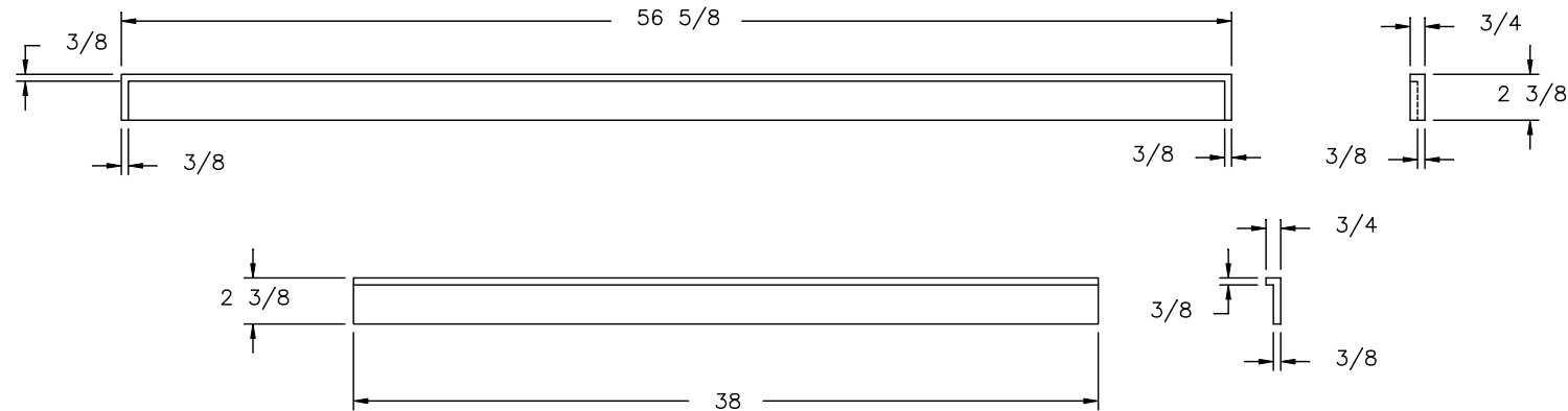
VINYL WRAP DETAILS – OUTER EDGE OF DETAIL B 2 EACH REQUIRED
