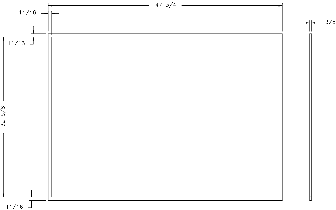
SPACERS DETAIL A TO DETAIL B
