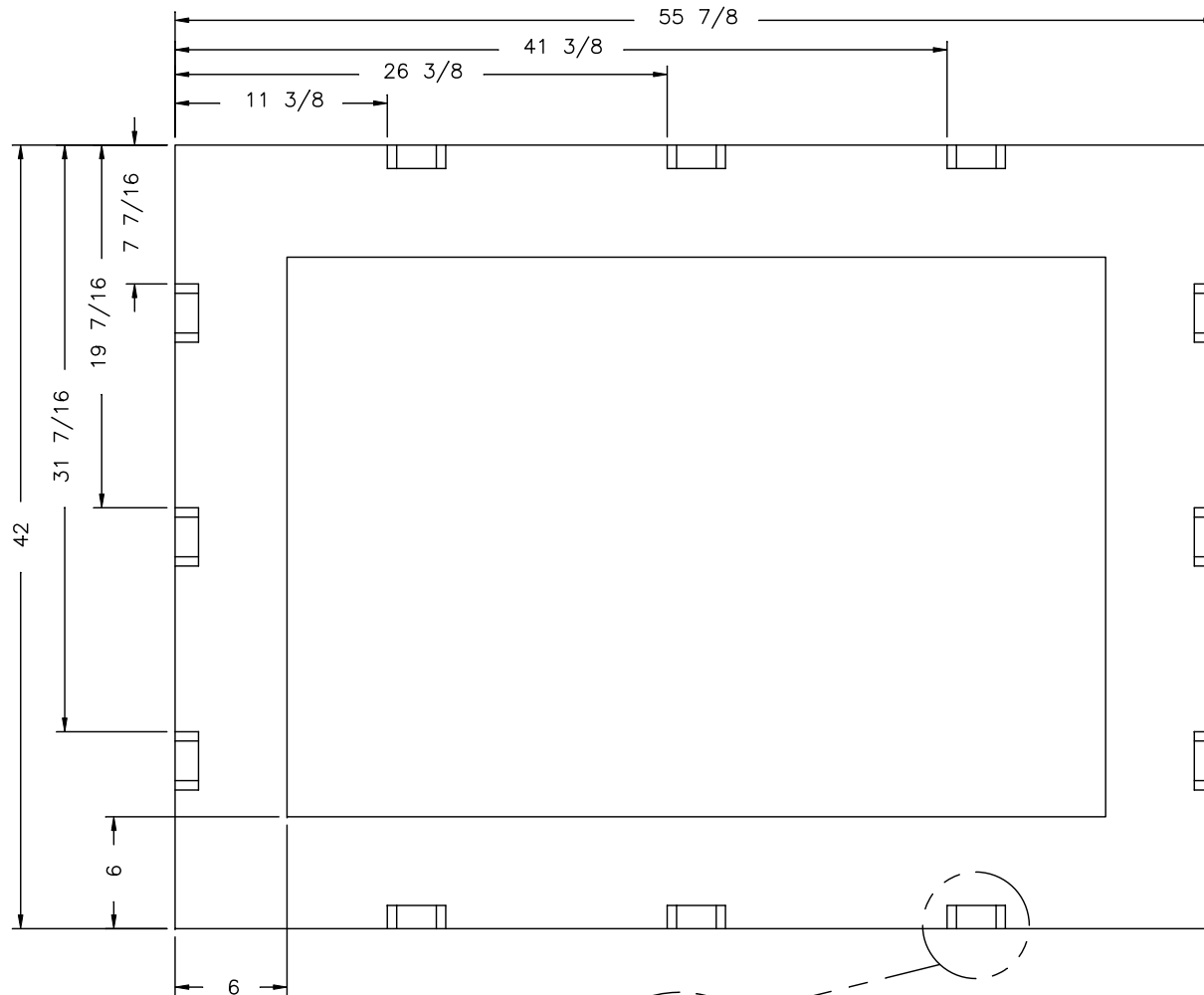
DETAIL B 3/8" PLYWOOD
