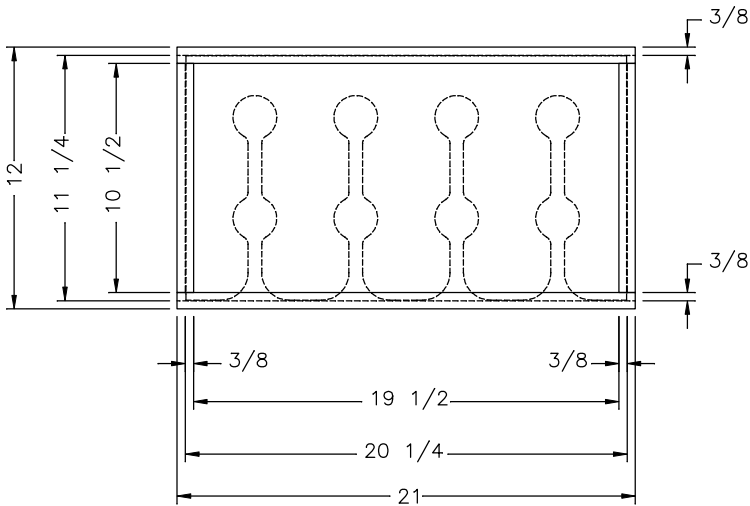
ASSEMBLY VIEWS
