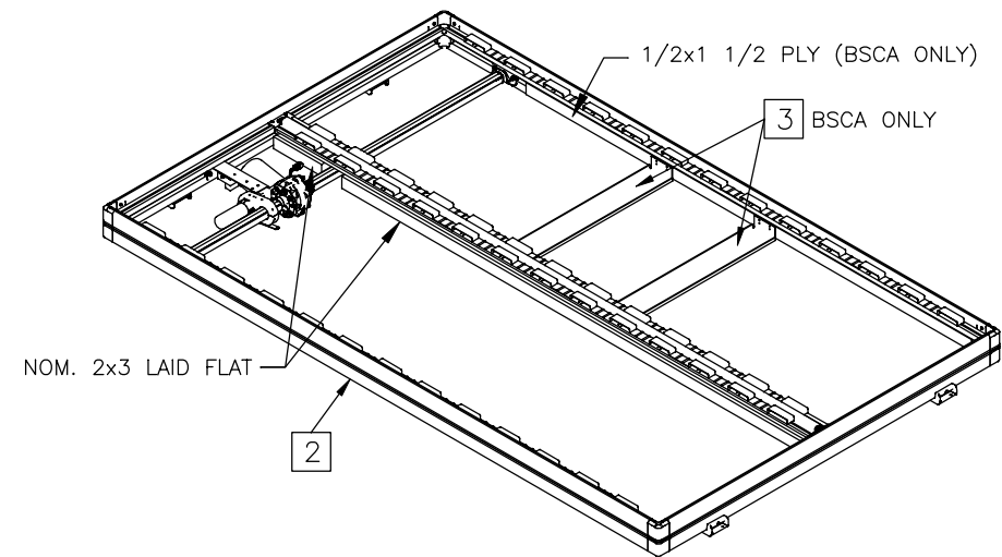
FRAME PREP ISO (SEE SHT. 2)
