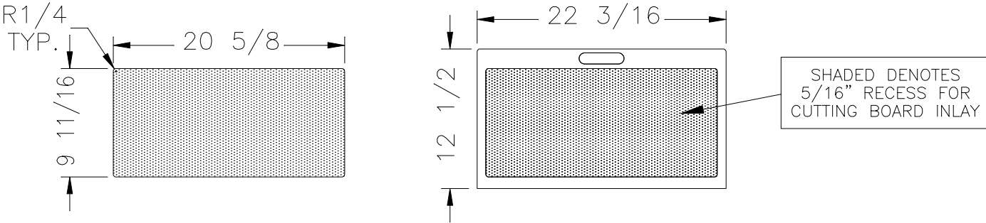
LID/CUTTING BOARD (2 REQ'D)
