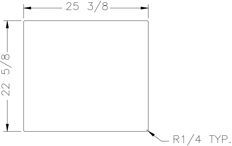
COUNTERTOP CUTOUT DETAIL
