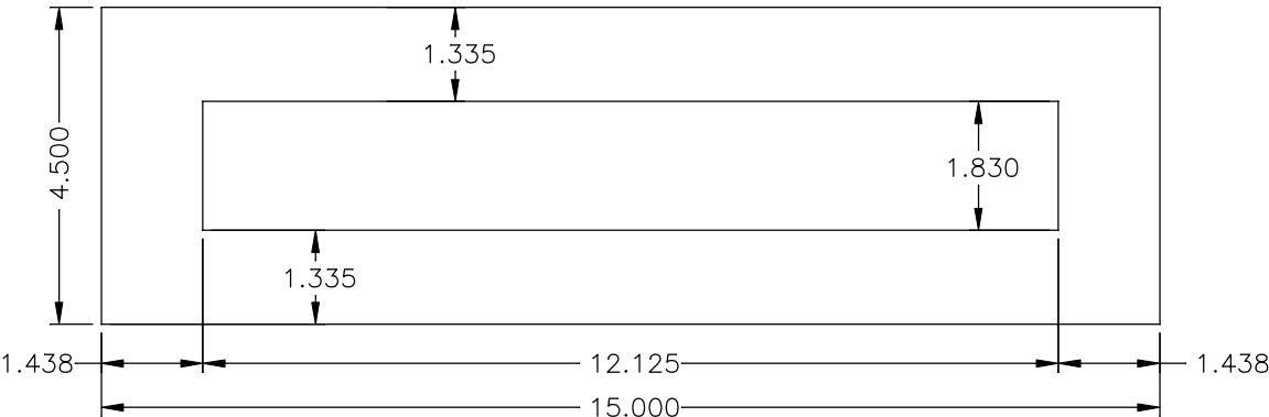
COLLAR FLAT PATTERN VIEW
