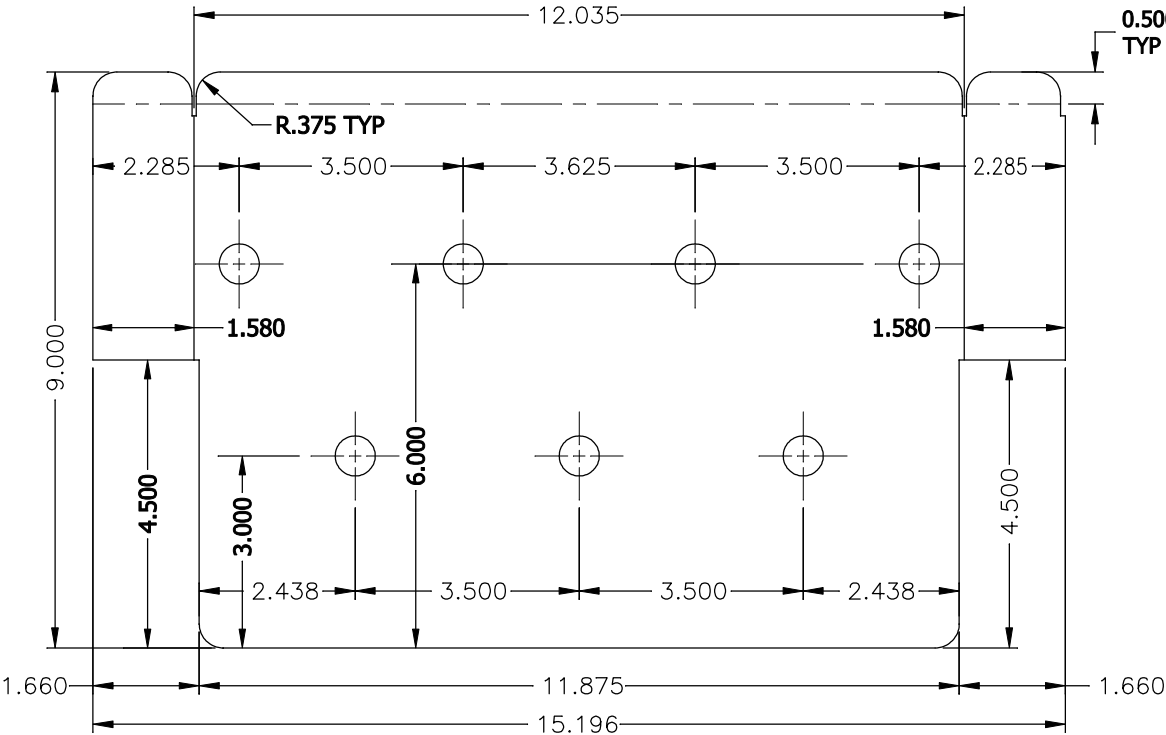
PLENUM, TOP, FLAT PATTERN
