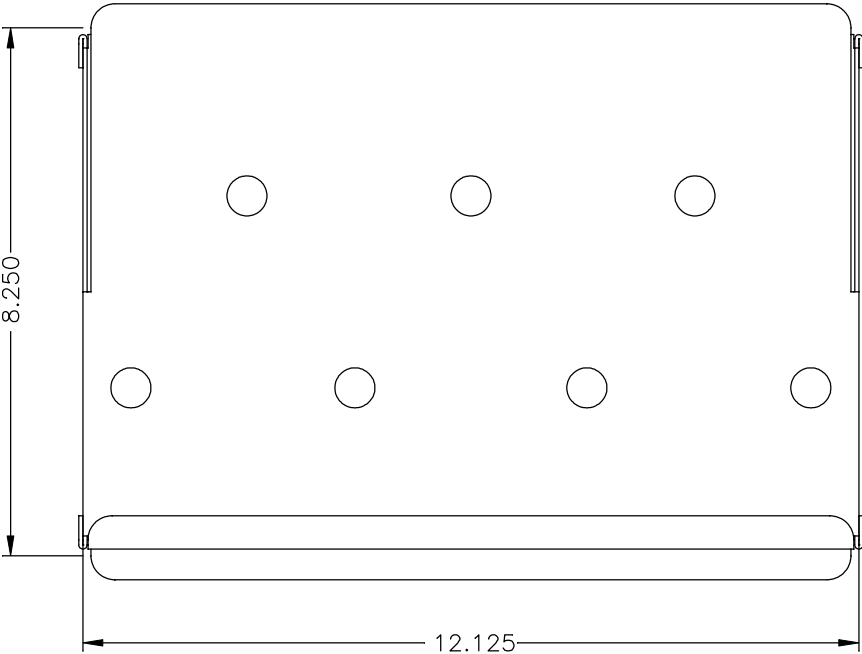
PLENUM, ASSEMBLED VIEW, TOP
