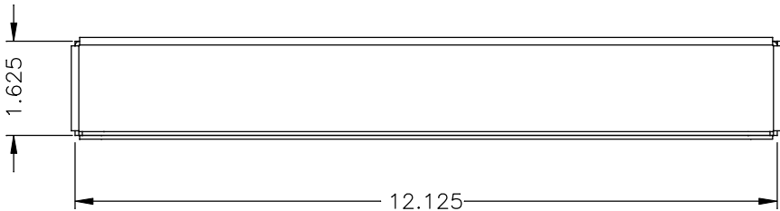
PLENUM, ASSEMBLED VIEW, END
