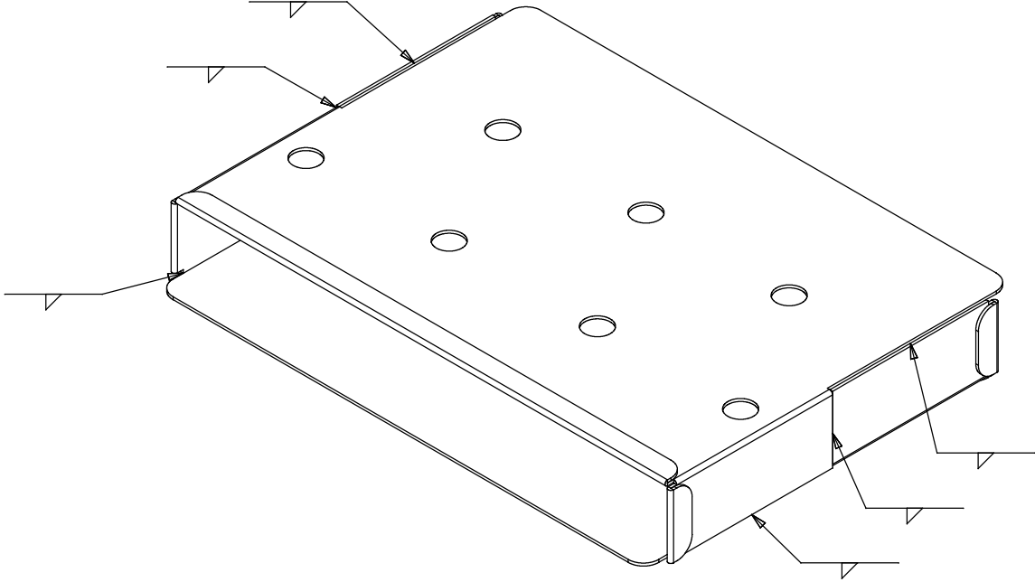
PLENUM, ASSEMBLED VIEW, ISO
