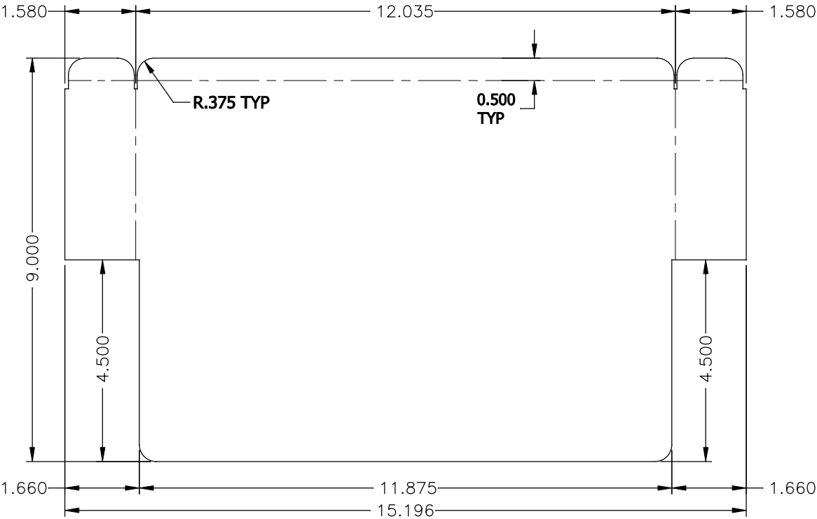
PLENUM, BOTTOM, FLAT PATTERN
