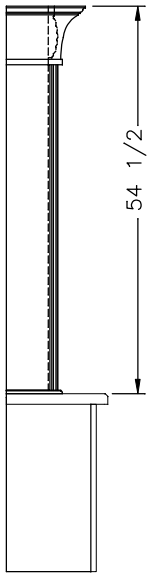
FASCIA RETURN FOR END TABLE
