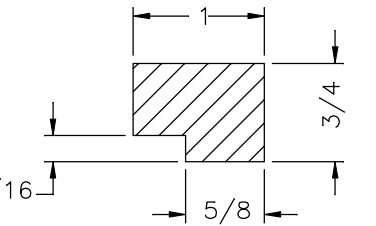
SECTION A-A 8X SCALE
