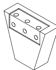
RECESS DETAIL (BACK & TOP)
