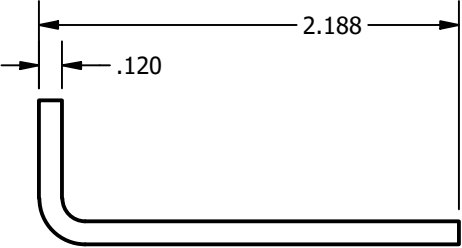
BENT END VIEW ITEM #4
