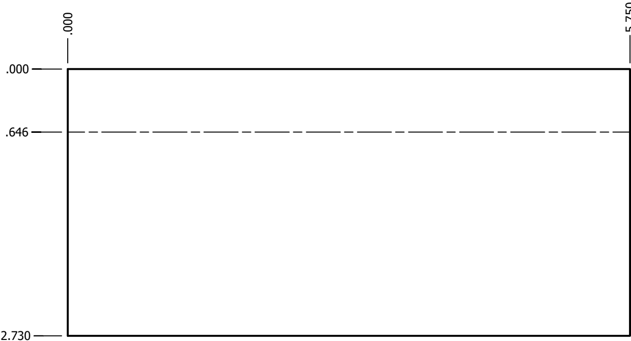
FLAT PATTERN ITEM #4
