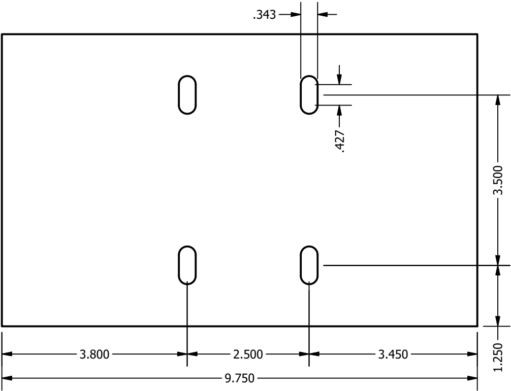
TOP VIEW ITEM #1
