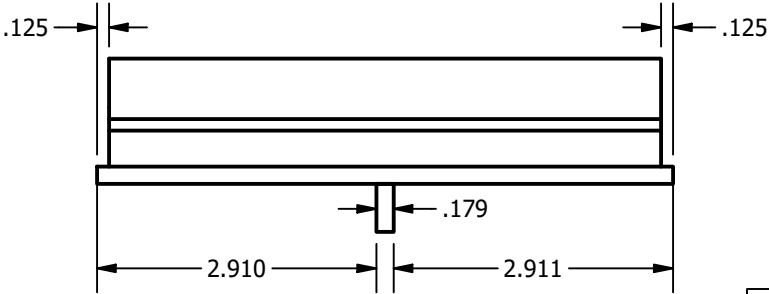
ASSEMBLY END VIEW
