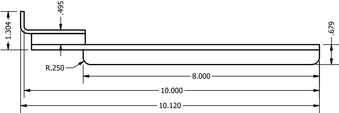
ASSEMBLY SIDE VIEW
