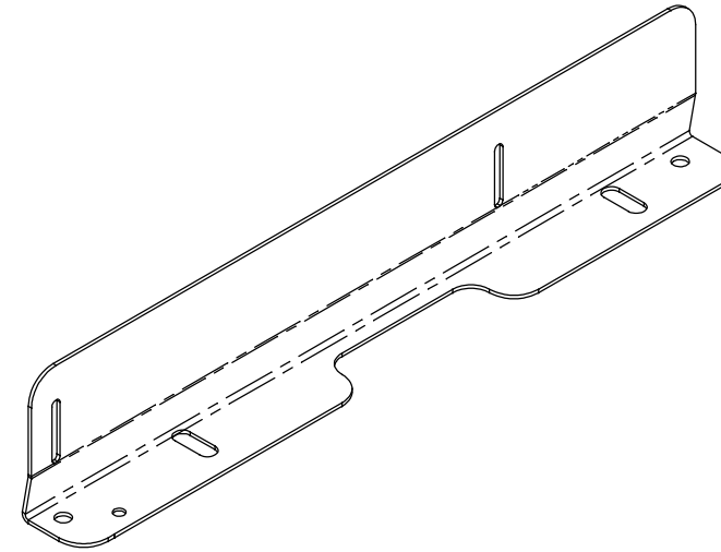
ISO VIEW
