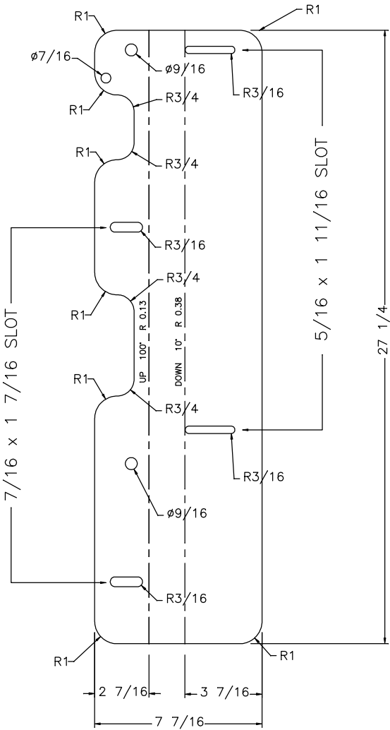
FLAT PATTERN
