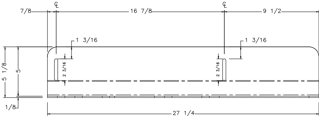
FRONT VIEW
