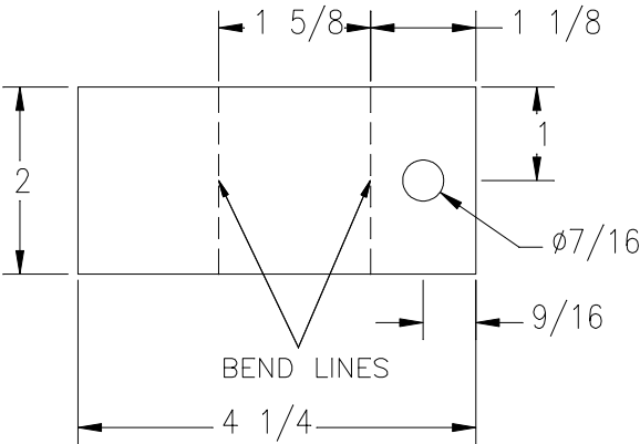
FLAT PATTERN
