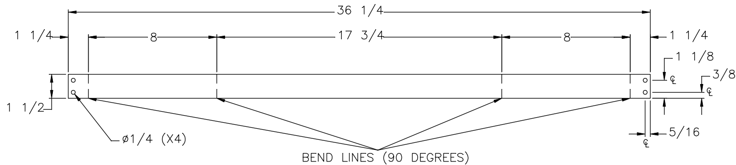
FLAT PATTERNS
