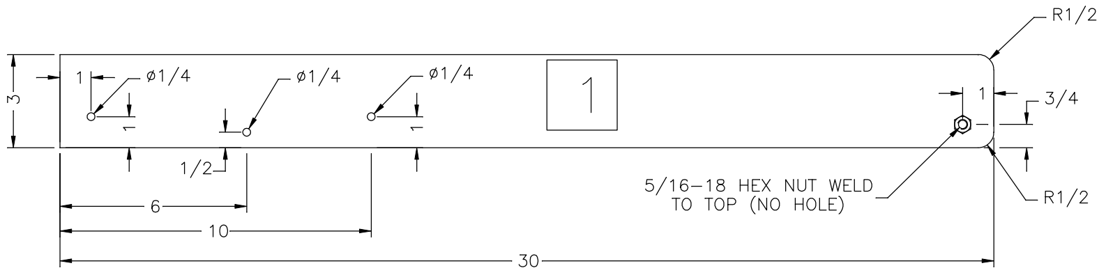
LEFT BRACKET
