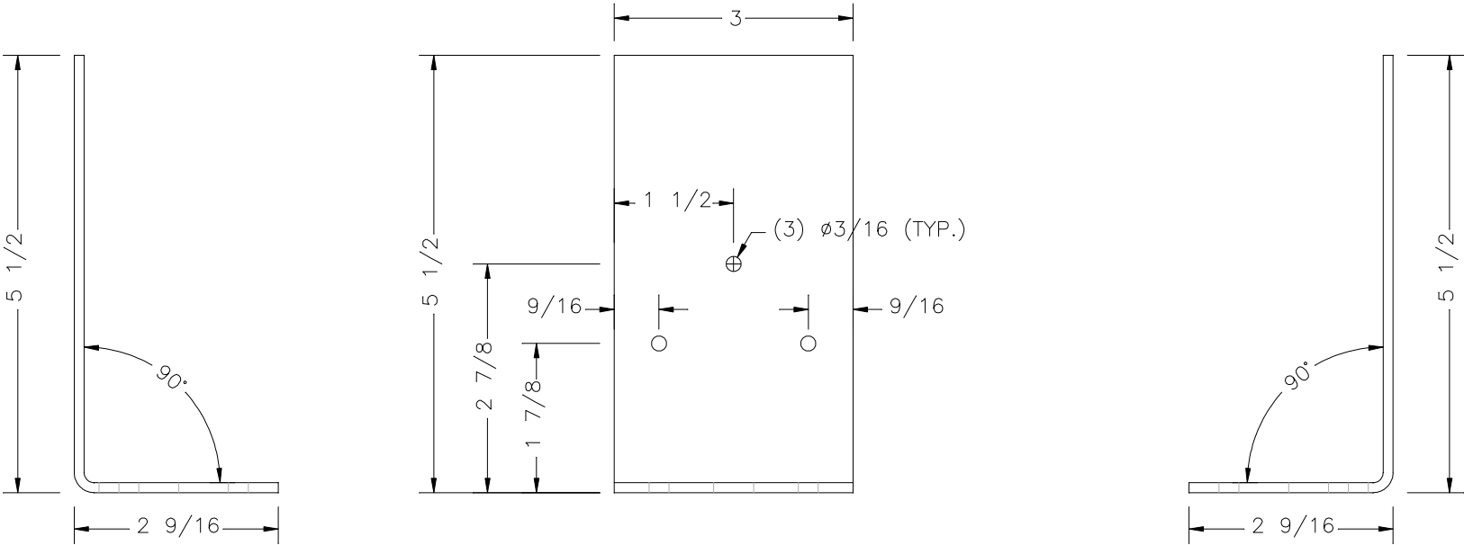
FRONT VIEW
