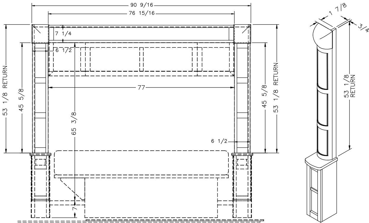
FASCIA RETURN DETAIL
