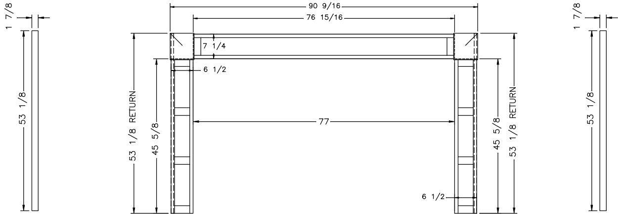
3/4" FASCIA RETURN DETAIL
