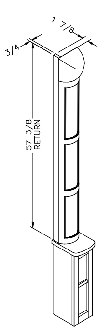
FASCIA RETURN DETAIL
