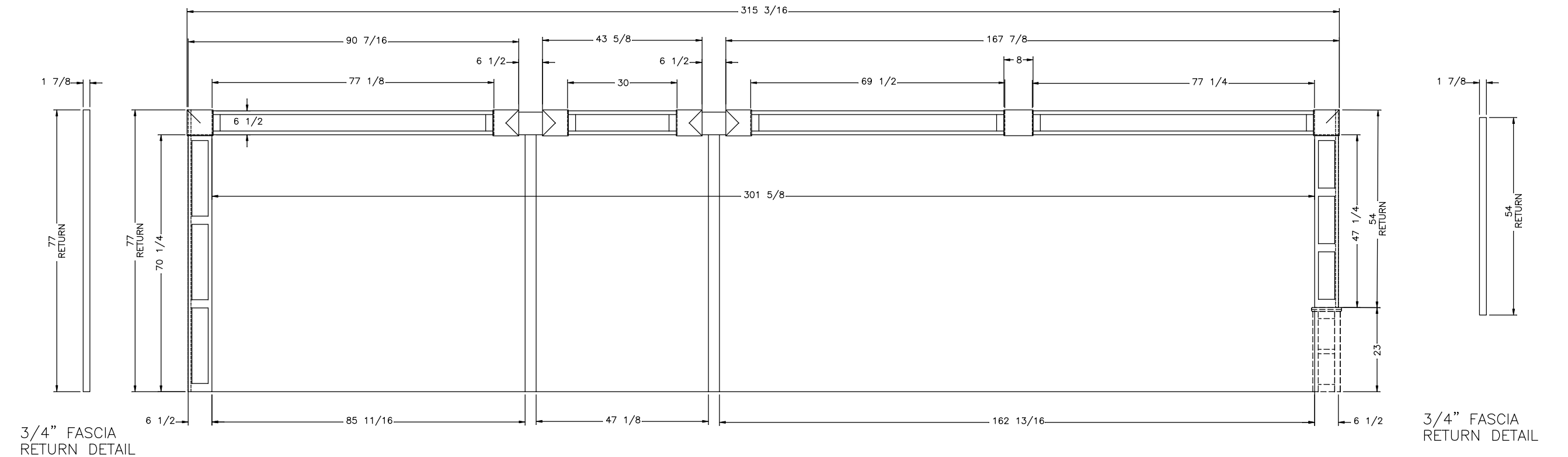
BR DRESSER/LIVINGROOM S-O FASCIA
