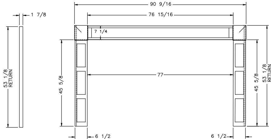
3/4" FASCIA RETURN DETAIL
