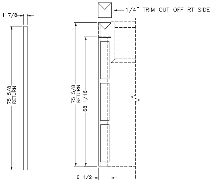
3/4" FASCIA RETURN DETAIL KITCHEN AREA S-O FASCIA
