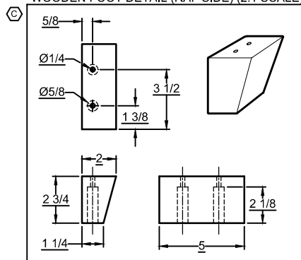
*WOODEN FOOT DETAIL (RAF SIDE) (2:1 SCALE)
