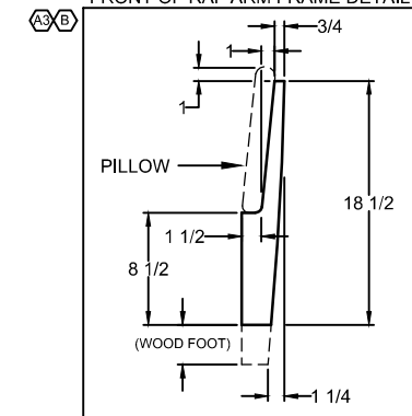
*FRONT OF RAF ARM FRAME DETAIL
