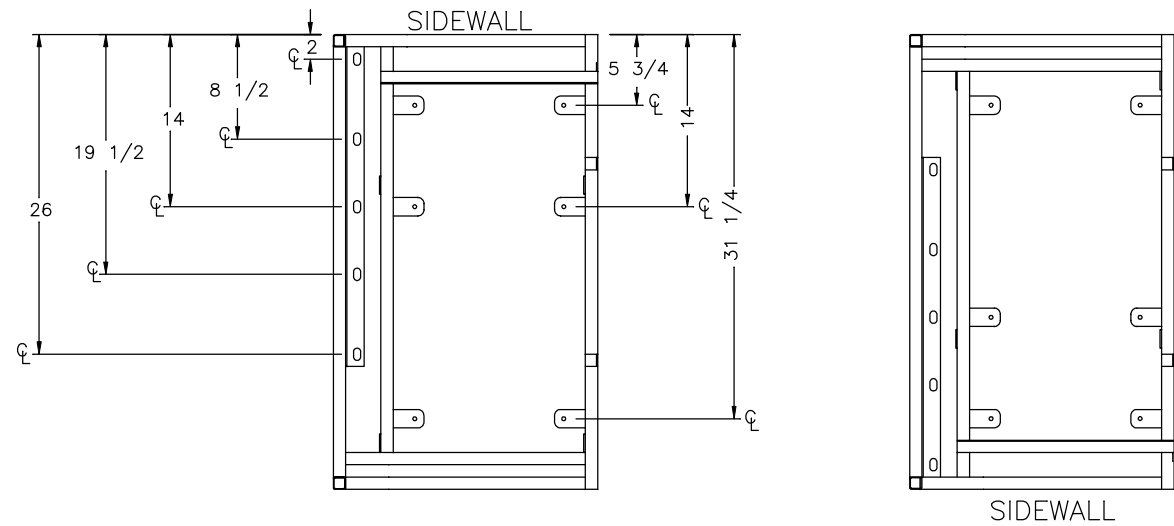
OFF DOOR SIDE(DRIVER SIDE) APPLICATION
