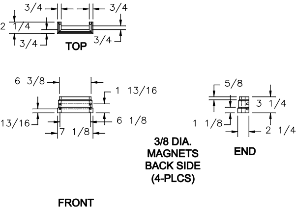
HWH FLAT FLOOR REMOVEABLE FOOT
