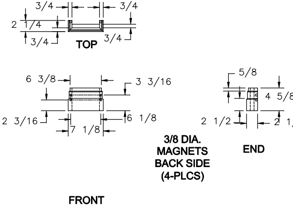
HWH NON FLAT FLOOR REMOVEABLE FOOT
