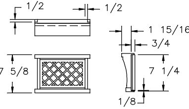
DIVIDER BLOCK
