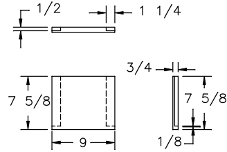
DIVIDER BLOCK
