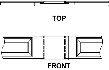
TYPICAL POCKET DOOR JAMB CONFIGURATION
