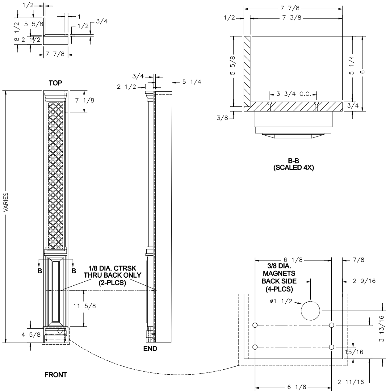
HWH NON-FLAT FLOOR COLUMN (LEFT/RIGHT REQ'D)
