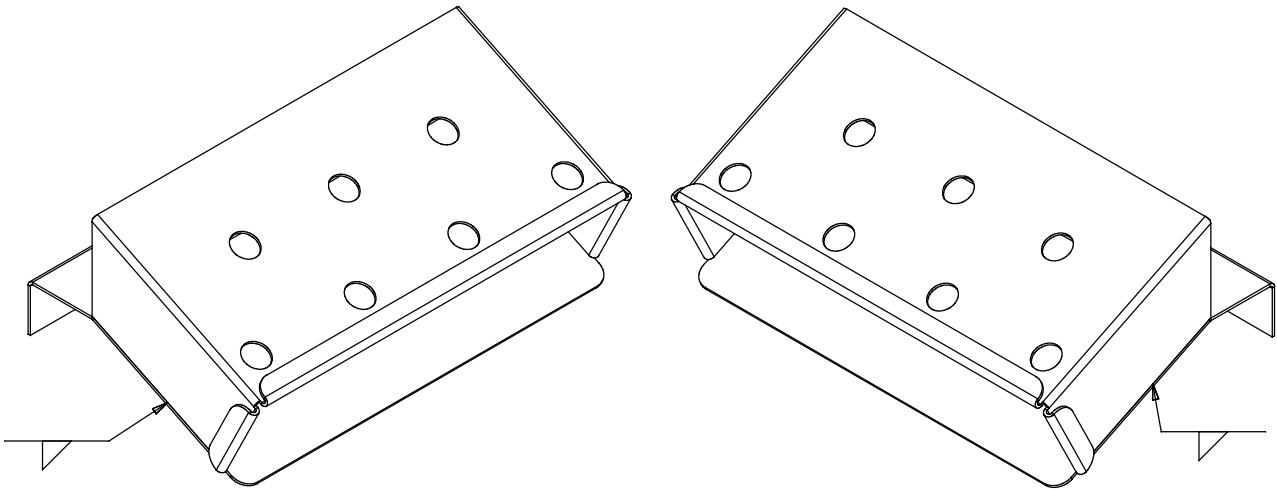
ISO VIEW
