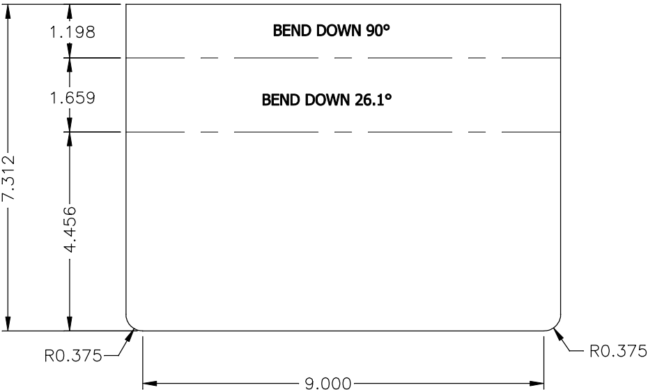
FLAT PATTERN
