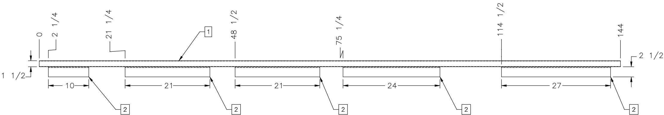
TOP VIEW
